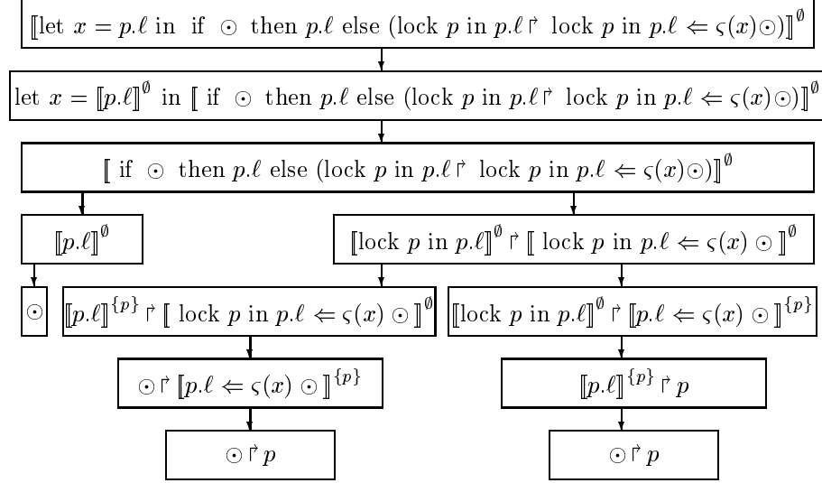
Figure 1: Abstract reduction graph for \alpha_s(a_1)
